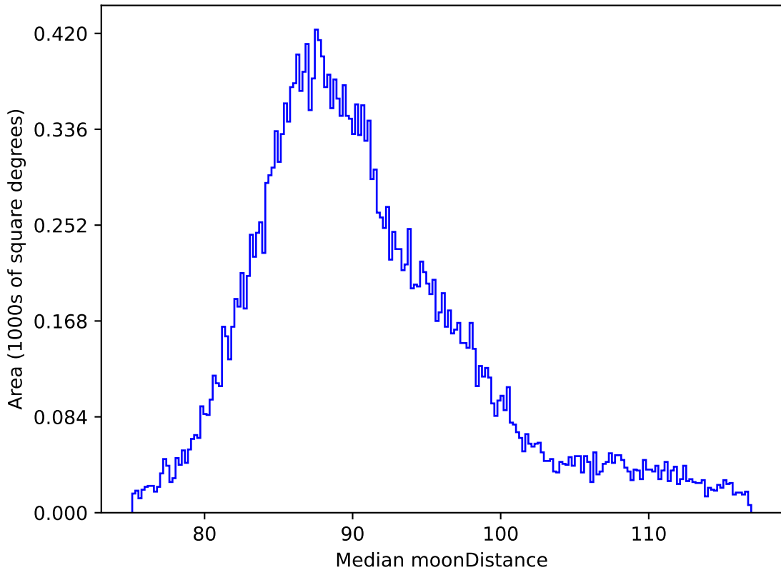
ddf_loaded_half_fl4_v3.4_10yrs All sky all bands: Median moonDistance
