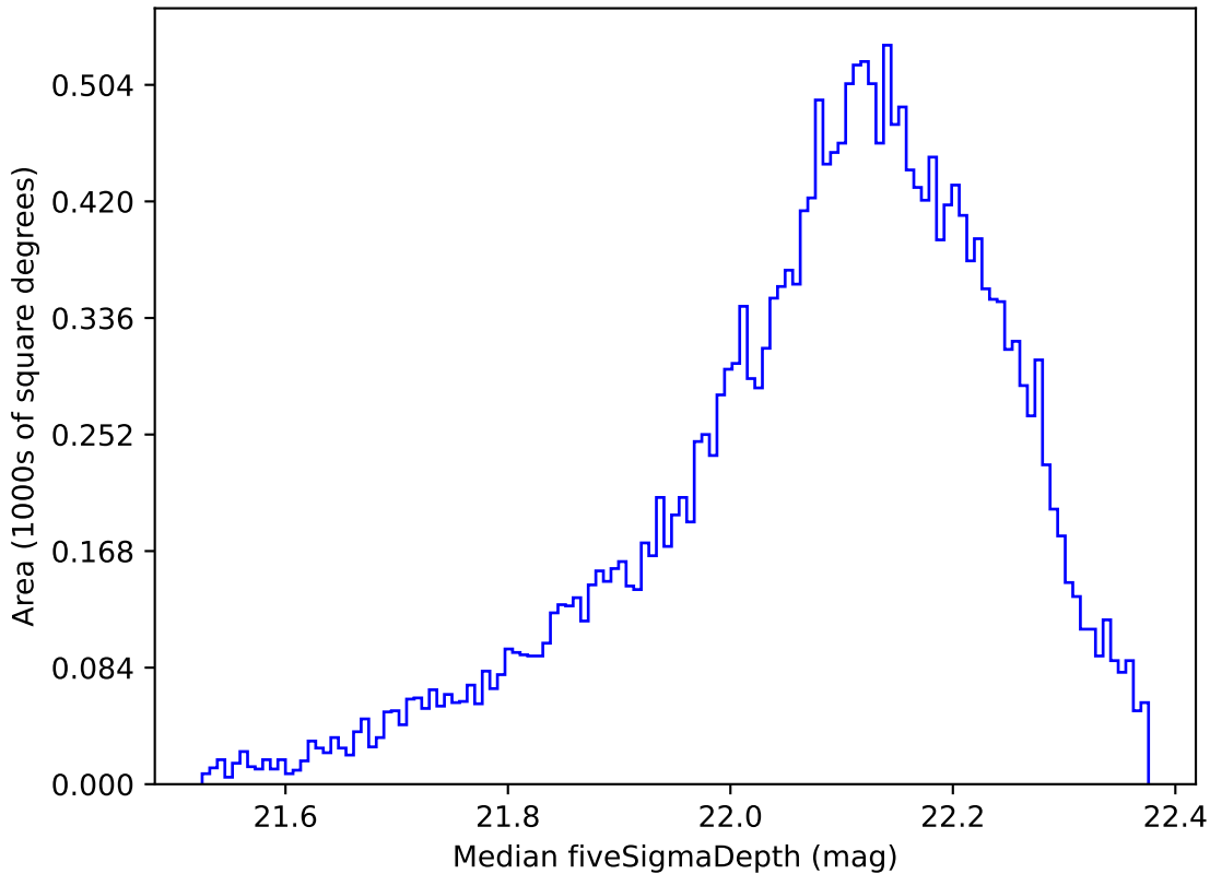
ddf_loaded_half_fl4_v3.4_10yrs Yr 1 y band: Median fiveSigmaDepth
