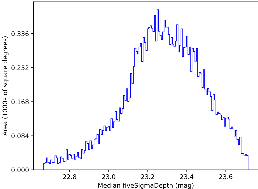
ddf_loaded_half_fl4_v3.4_10yrs Yr 1 u band: Median fiveSigmaDepth
