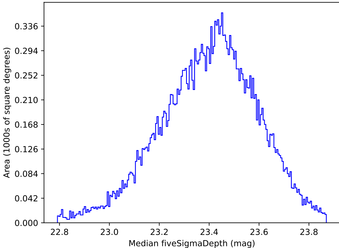
ddf_loaded_half_fl4_v3.4_10yrs Yr 1 all bands: Median fiveSigmaDepth
