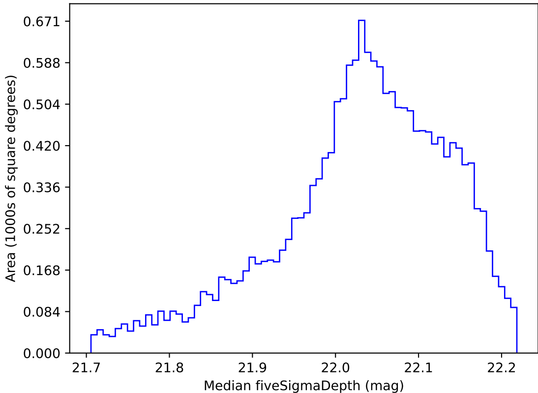
ddf_loaded_half_fl4_v3.4_10yrs WFD y band: Median fiveSigmaDepth
