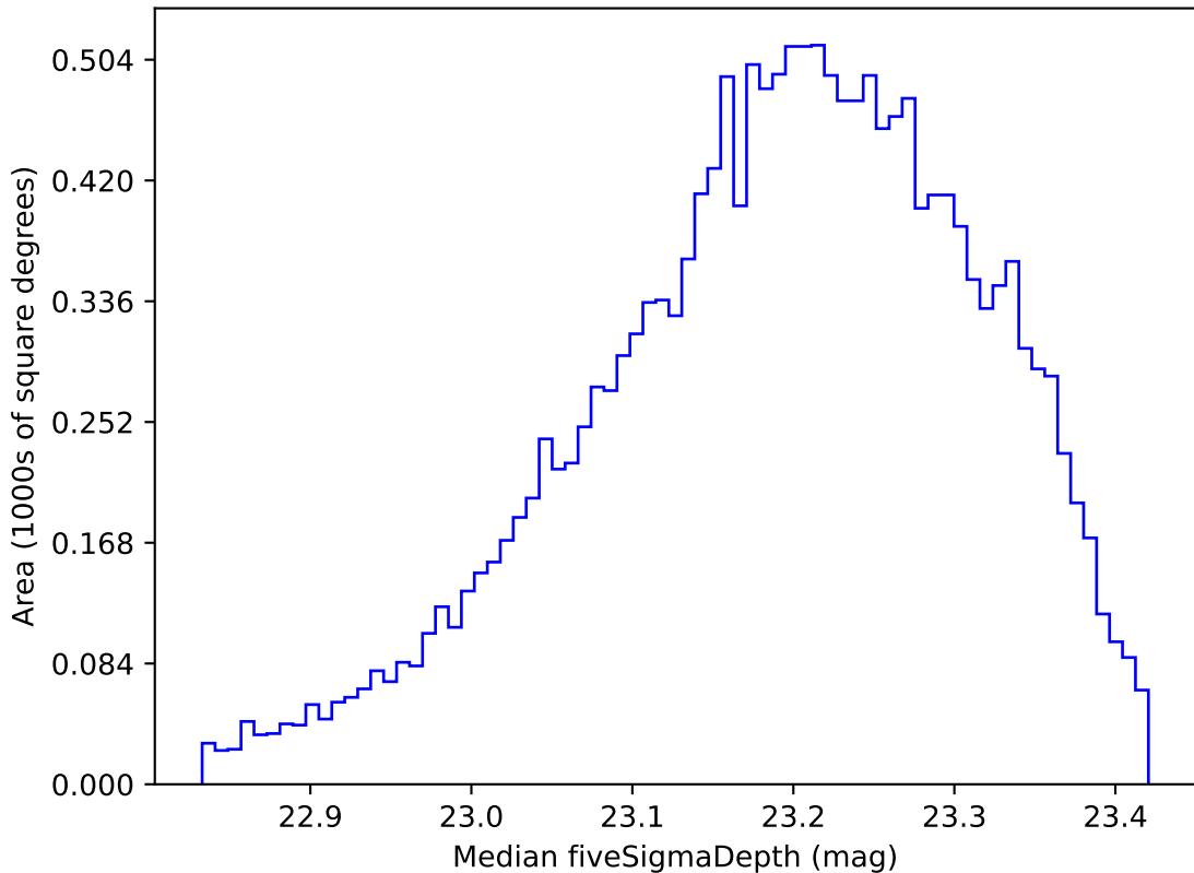
ddf_loaded_half_fl4_v3.4_10yrs WFD u band: Median fiveSigmaDepth
