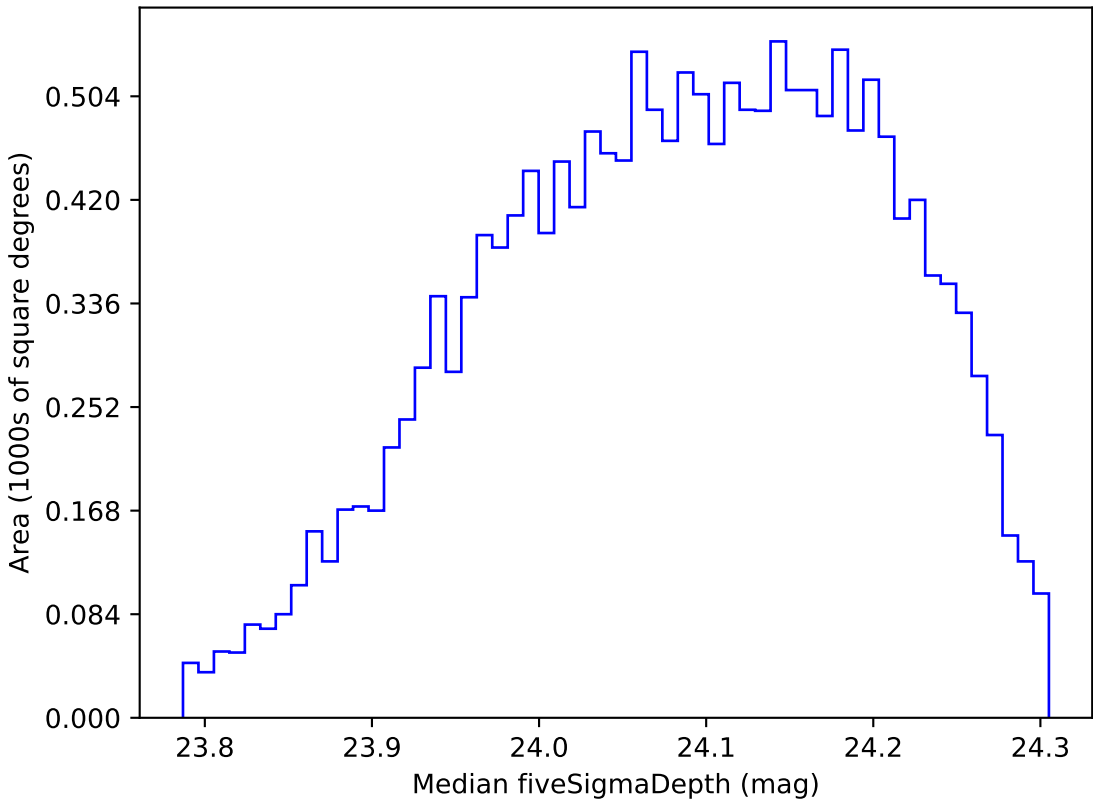
ddf_loaded_half_fl4_v3.4_10yrs WFD r band: Median fiveSigmaDepth
