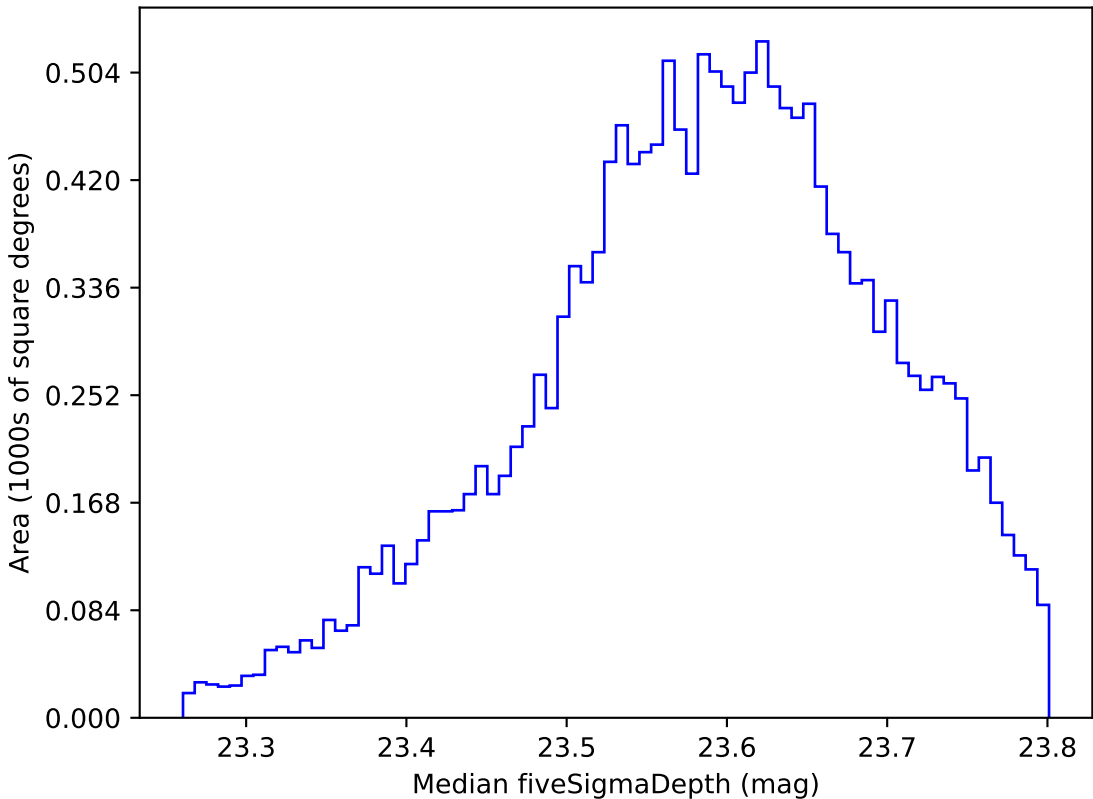
ddf_loaded_half_fl4_v3.4_10yrs WFD i band: Median fiveSigmaDepth
