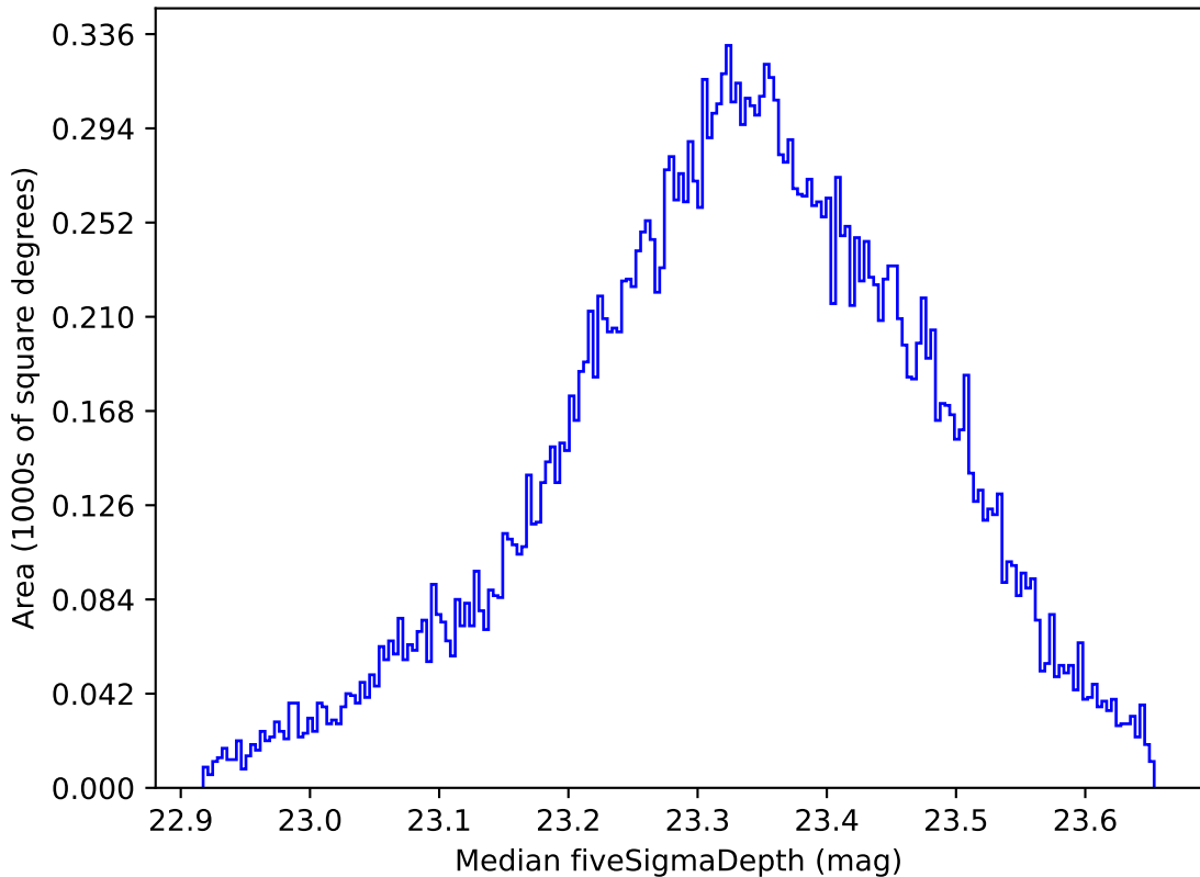
ddf_loaded_half_fl4_v3.4_10yrs All sky all bands: Median fiveSigmaDepth
