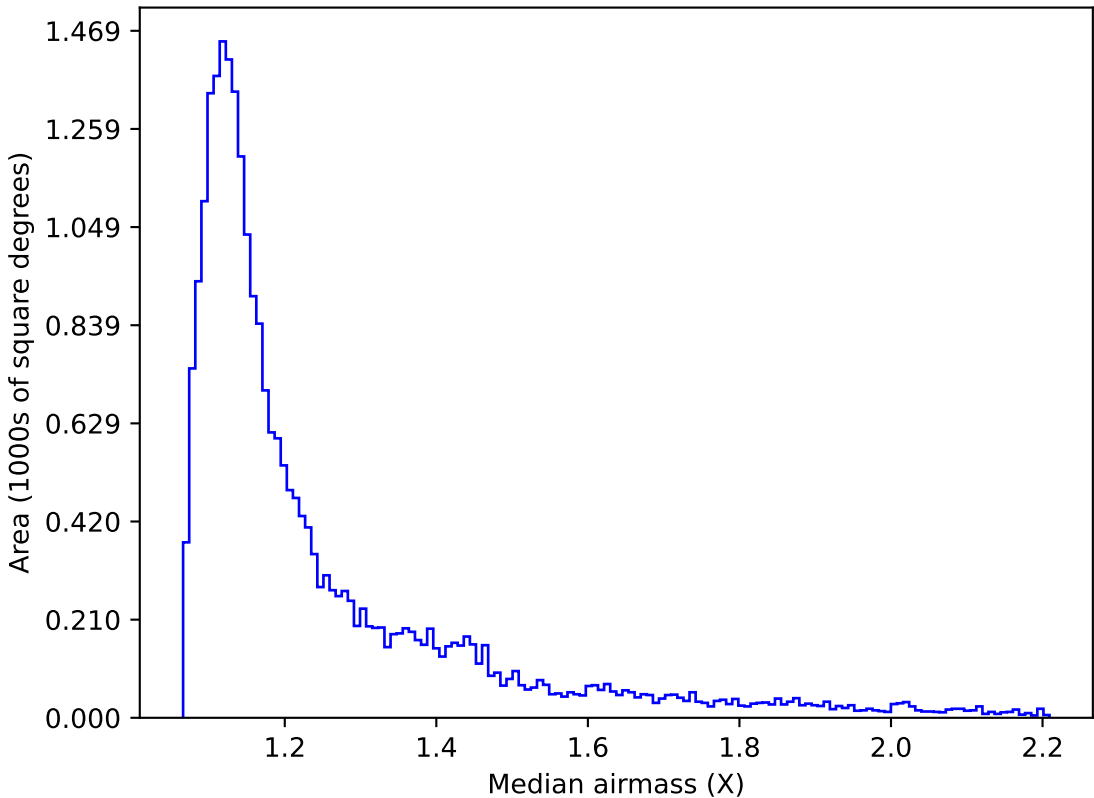
ddf_loaded_half_fl4_v3.4_10yrs Yr 1 z band: Median airmass
