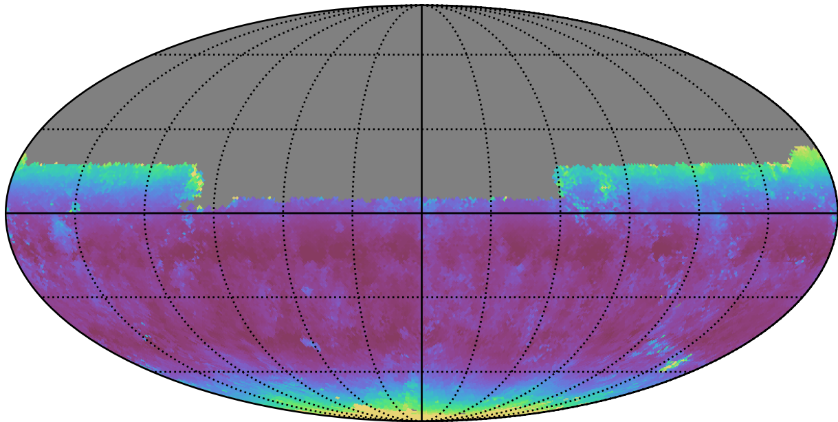
ddf_loaded_half_fl4_v3.4_10yrs Yr 1 y band: Median airmass
