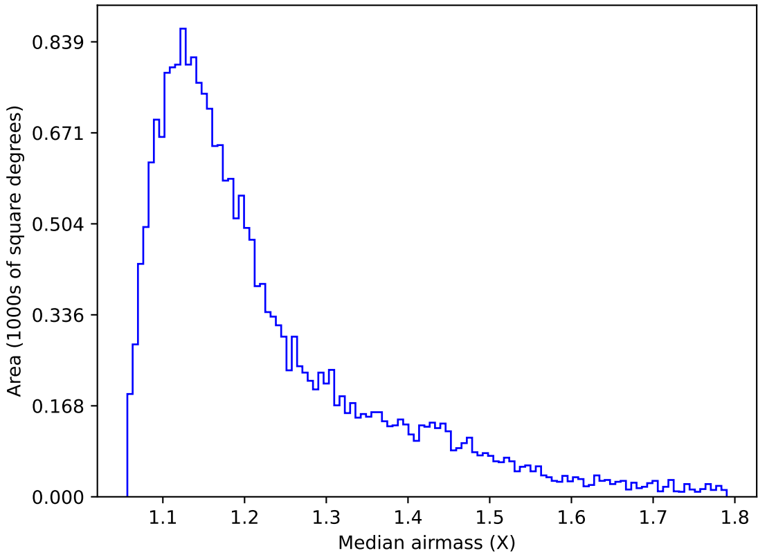
ddf_loaded_half_fl4_v3.4_10yrs Yr 1 u band: Median airmass
