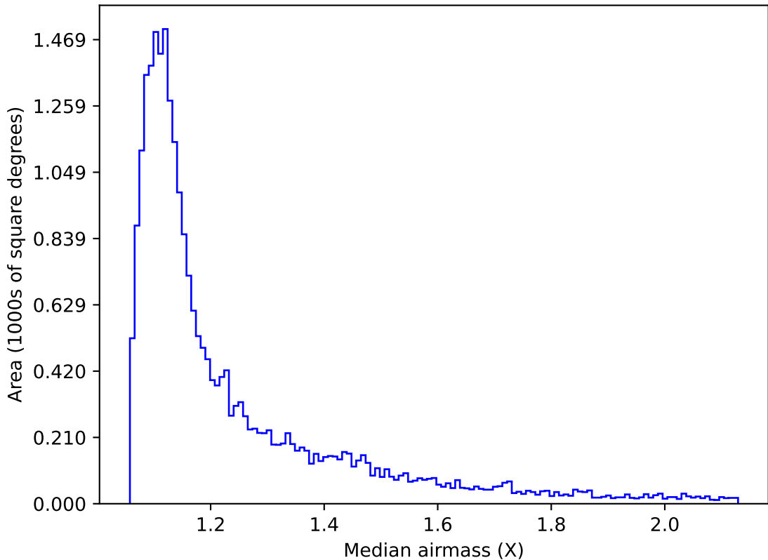
ddf_loaded_half_fl4_v3.4_10yrs Yr 1 r band: Median airmass
