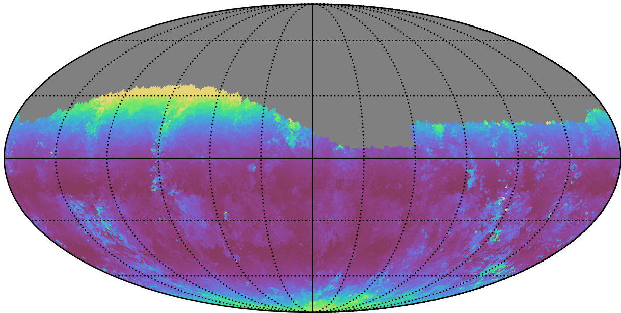
ddf_loaded_half_fl4_v3.4_10yrs Yr 1 g band: Median airmass
