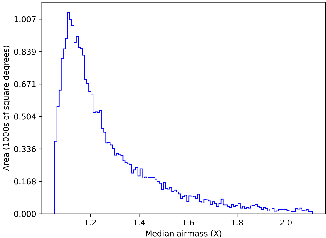
ddf_loaded_half_fl4_v3.4_10yrs Yr 1 g band: Median airmass
