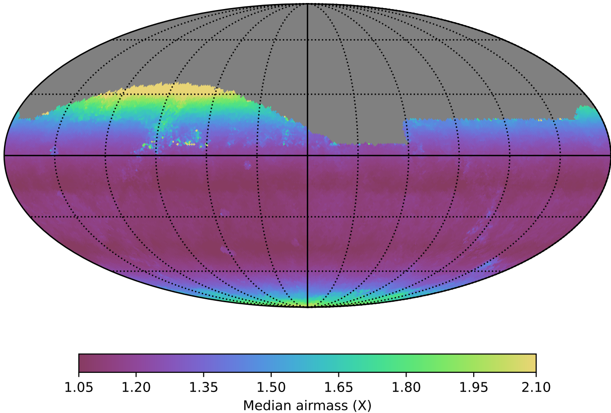
ddf_loaded_half_fl4_v3.4_10yrs Yr 1 all bands: Median airmass
