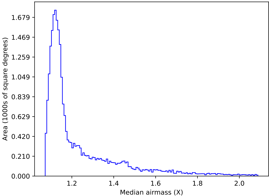
ddf_loaded_half_f14_v3.4_10yrs Yr 1 all bands: Median airmass
