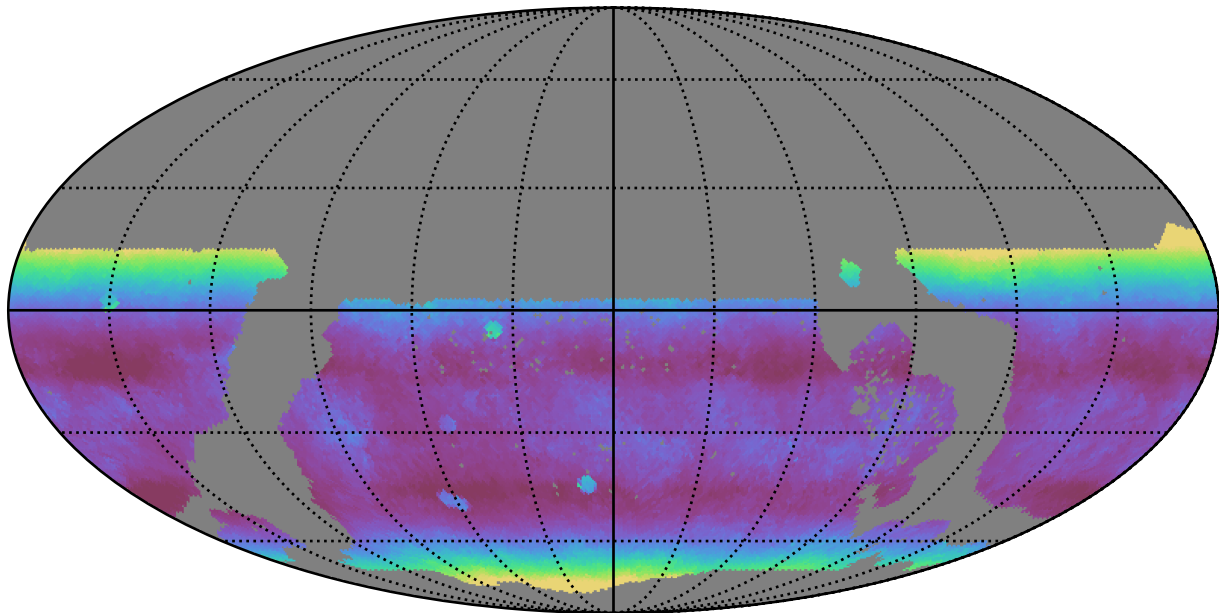
ddf_loaded_half_fl4_v3.4_10yrs WFD z band: Median airmass
