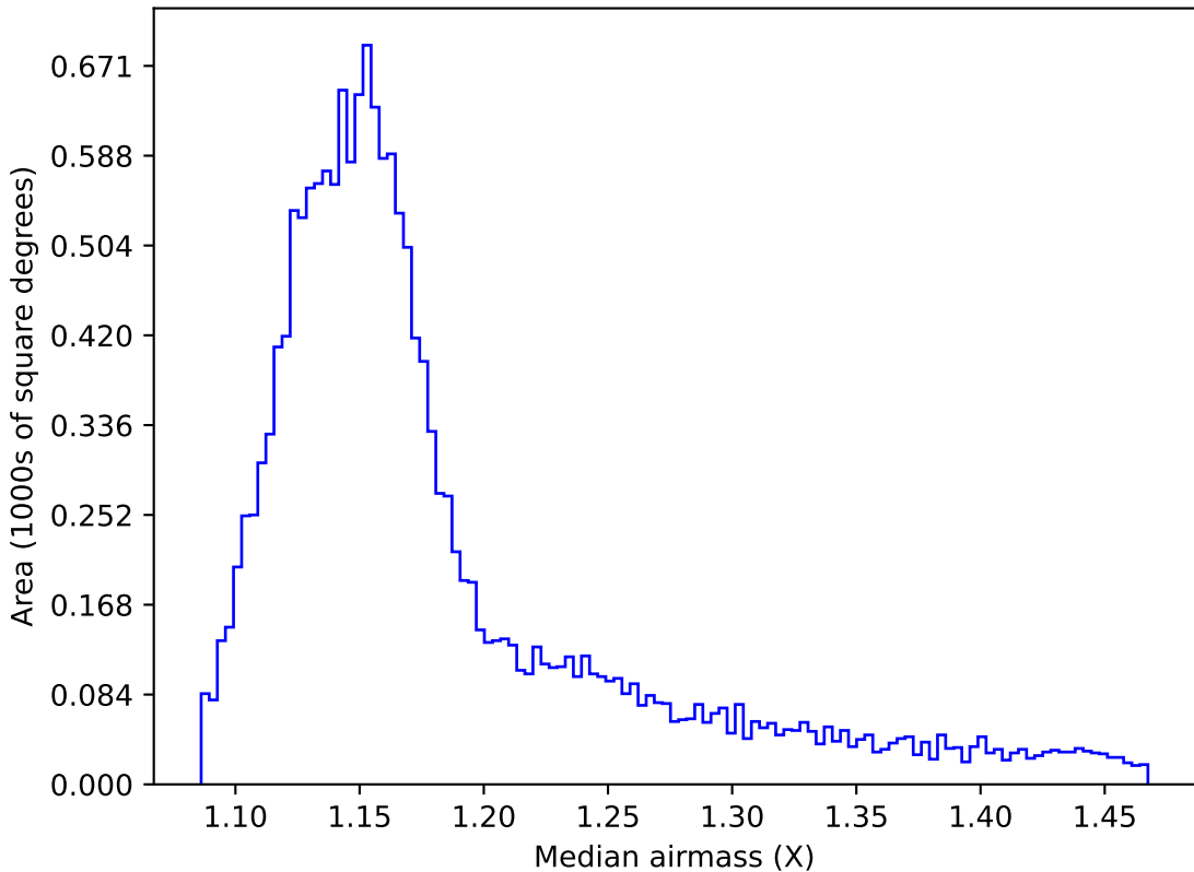
ddf_loaded_half_fl4_v3.4_10yrs WFD z band: Median airmass
