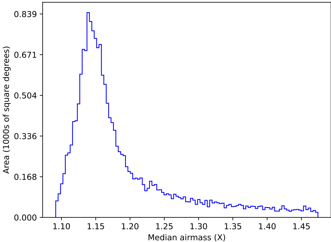
ddf_loaded_half_fl4_v3.4_10yrs WFD y band: Median airmass
