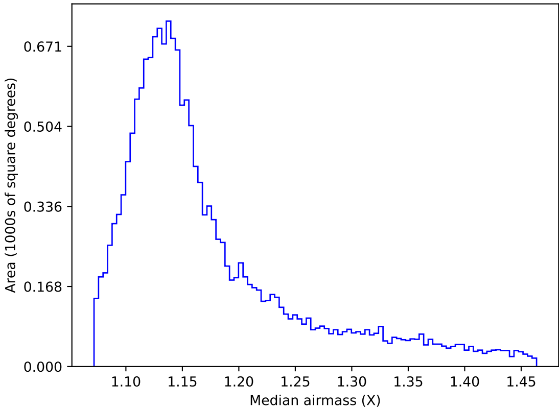
ddf_loaded_half_f14_v3.4_10yrs WFD u band: Median airmass
