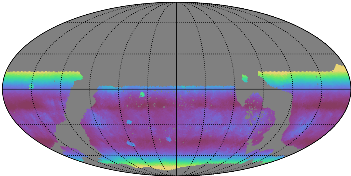
ddf_loaded_half_fl4_v3.4_10yrs WFD r band: Median airmass
