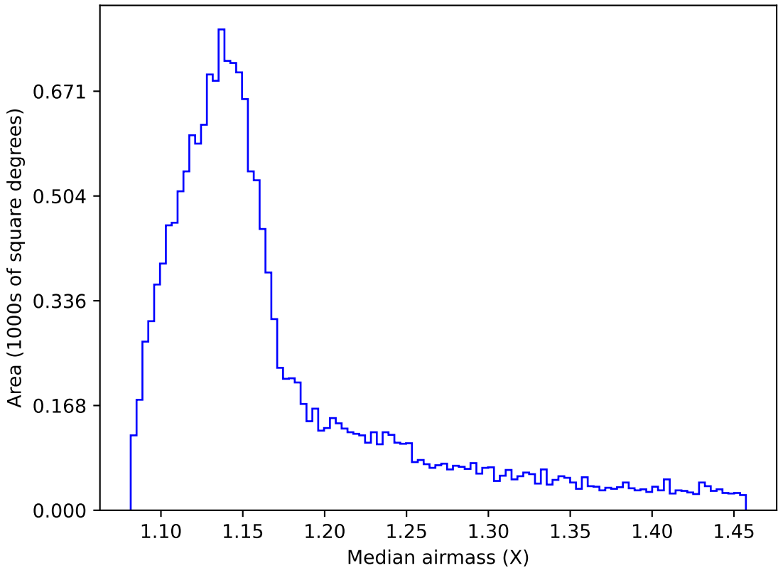
ddf_loaded_half_fl4_v3.4_10yrs WFD i band: Median airmass
