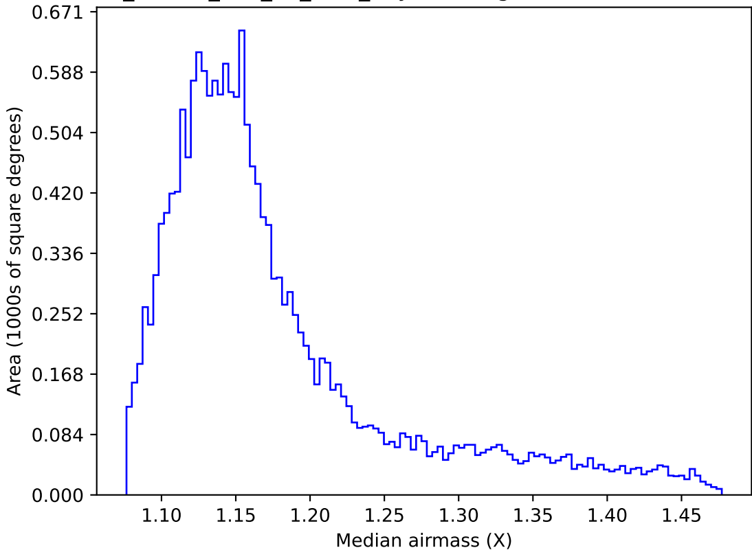
ddf_loaded_half_fl4_v3.4_10yrs WFD g band: Median airmass
