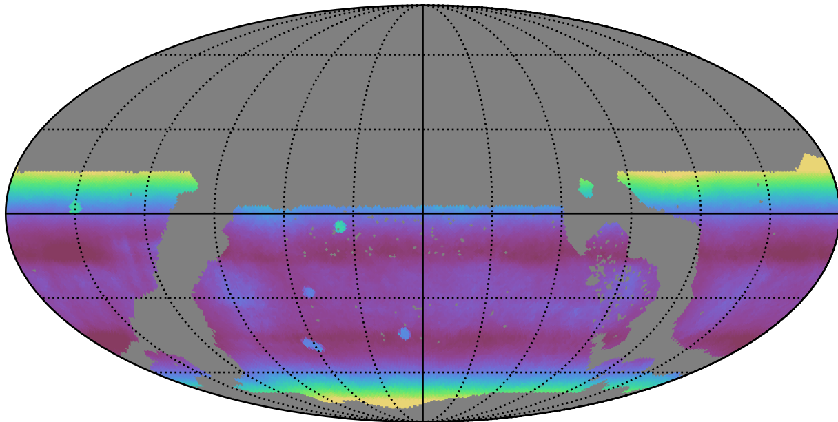
ddf_loaded_half_fl4_v3.4_10yrs WFD all bands: Median airmass
