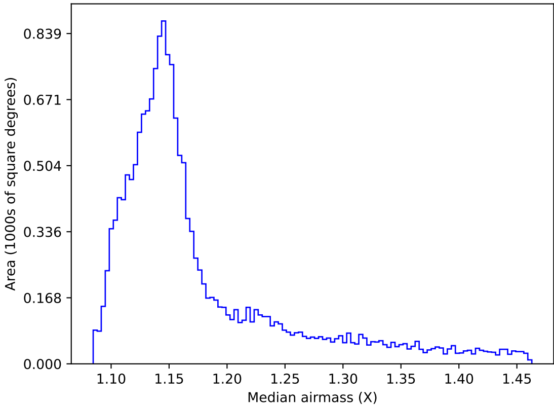
ddf_loaded_half_fl4_v3.4_10yrs WFD all bands: Median airmass
