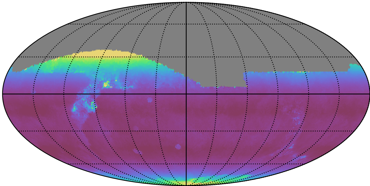
ddf_loaded_half_fl4_v3.4_10yrs All sky z band: Median airmass
