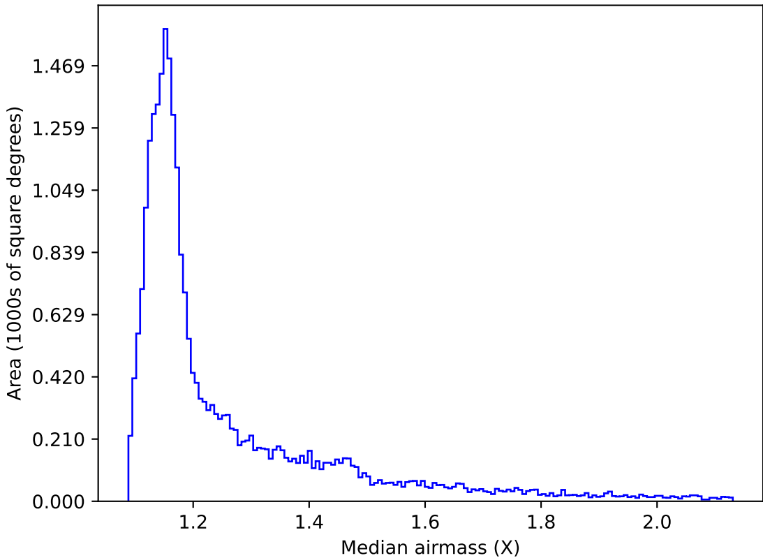
ddf_loaded_half_fl4_v3.4_10yrs All sky z band: Median airmass
