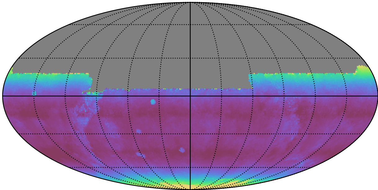
ddf_loaded_half_fl4_v3.4_10yrs All sky y band: Median airmass
