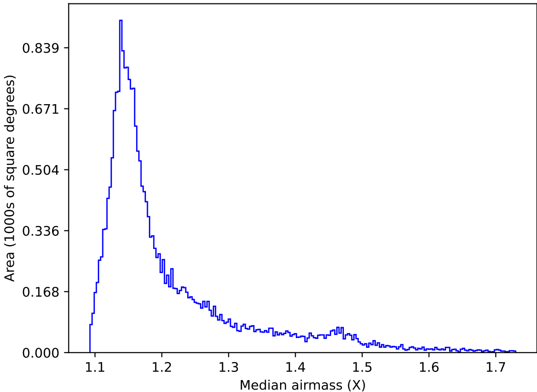
ddf_loaded_half_fl4_v3.4_10yrs All sky y band: Median airmass
