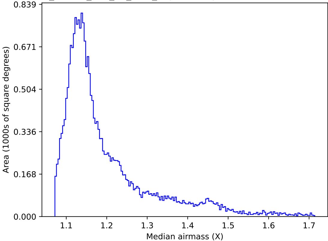
ddf_loaded_half_fl4_v3.4_10yrs All sky u band: Median airmass
