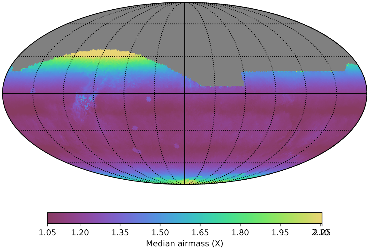
ddf_loaded_half_fl4_v3.4_10yrs All sky r band: Median airmass
