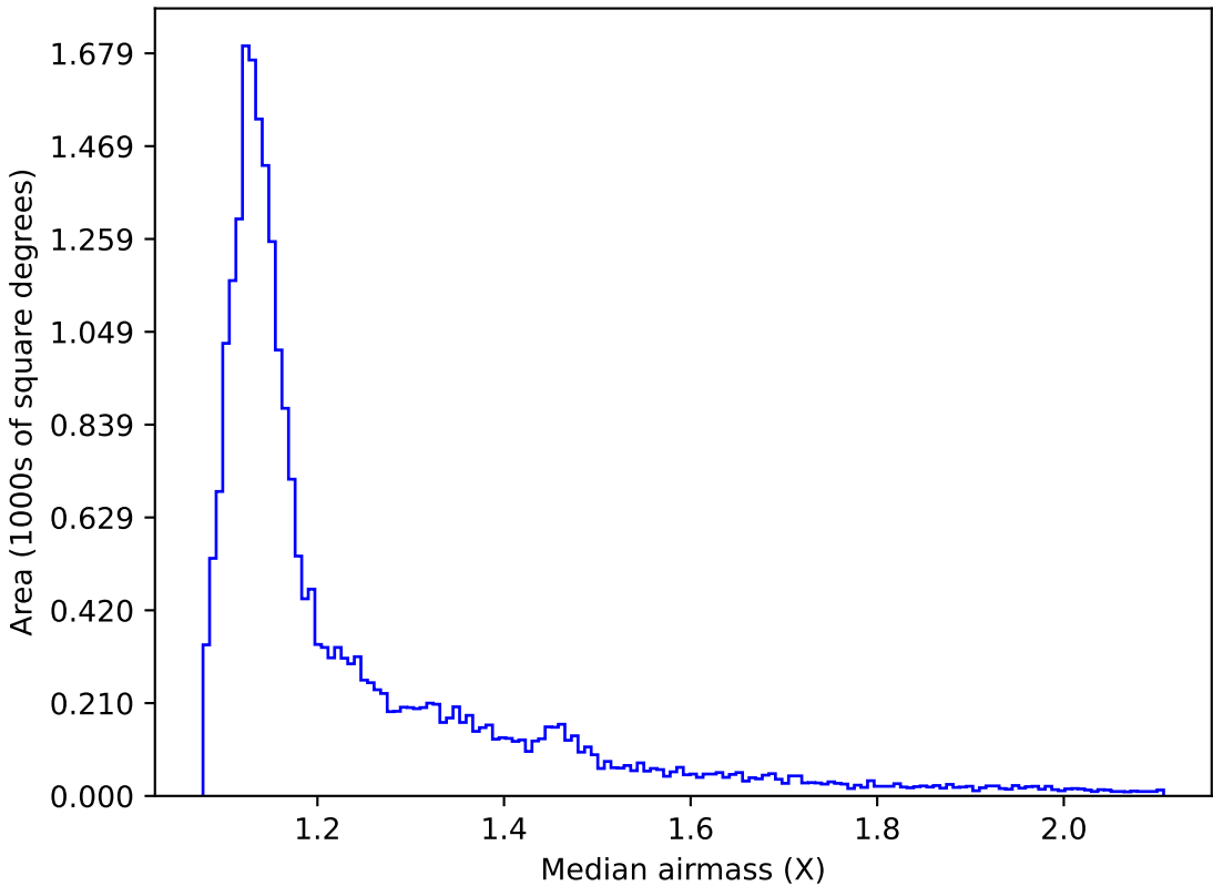
ddf_loaded_half_fl4_v3.4_10yrs All sky r band: Median airmass
