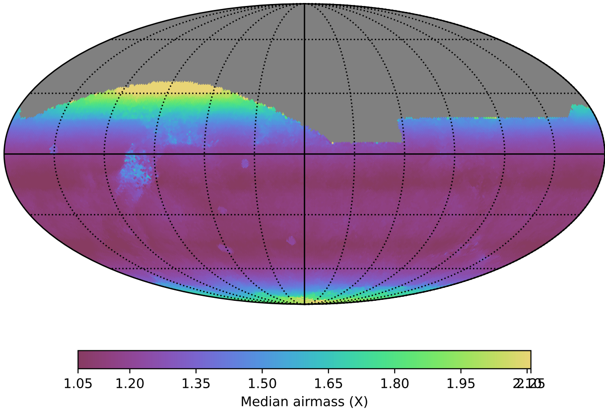
ddf_loaded_half_fl4_v3.4_10yrs All sky i band: Median airmass
