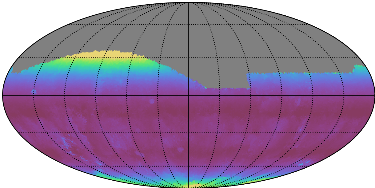
ddf_loaded_half_fl4_v3.4_10yrs All sky g band: Median airmass
