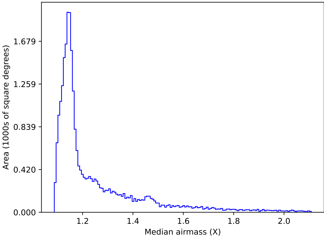
ddf_loaded_half_fl4_v3.4_10yrs All sky all bands: Median airmass
