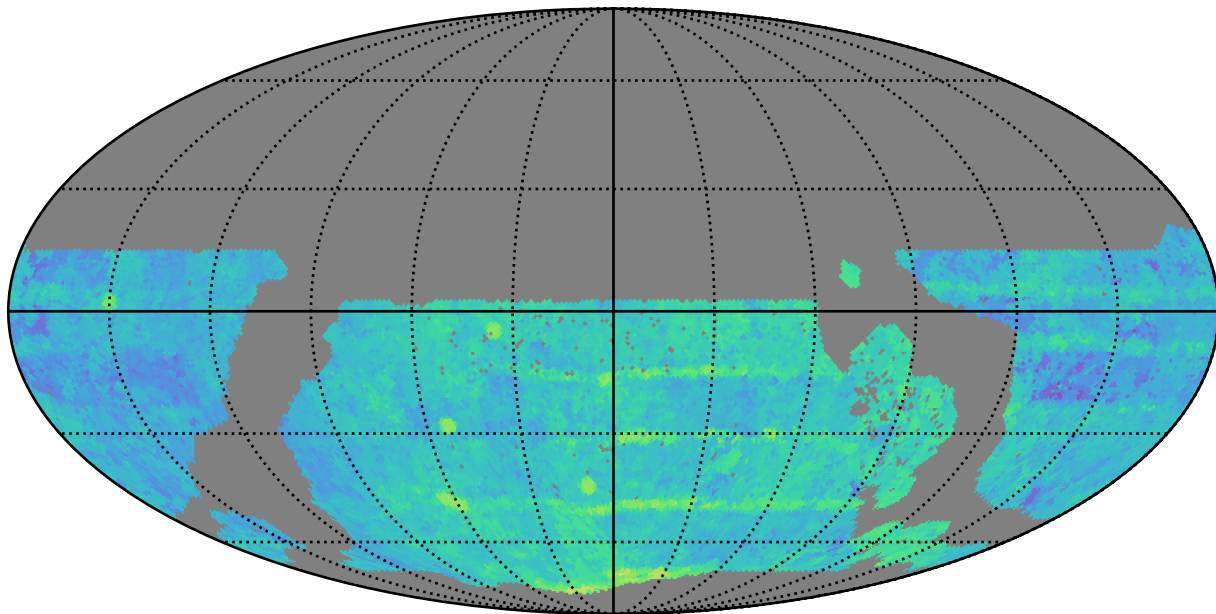
ddf_loaded_half_fl4_v3.4_10yrs WFD z band: Median Season Length
