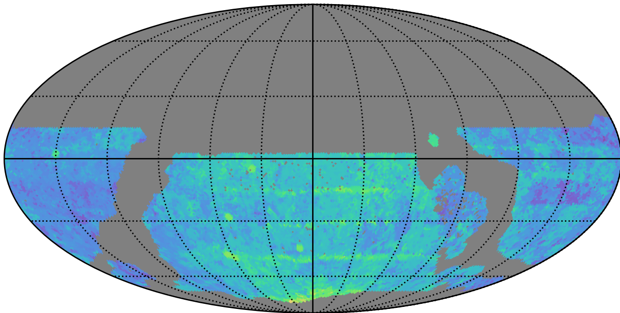
ddf_loaded_half_fl4_v3.4_10yrs WFD y band: Median Season Length
