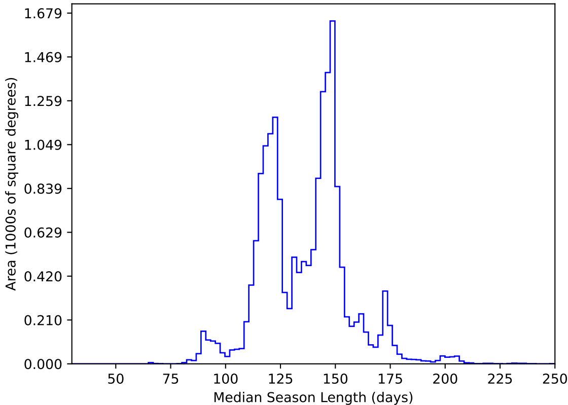
ddf_loaded_half_fl4_v3.4_10yrs WFD y band: Median Season Length
