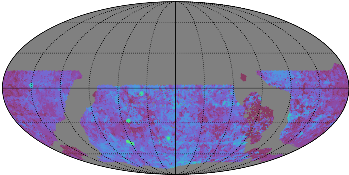
ddf_loaded_half_fl4_v3.4_10yrs WFD u band: Median Season Length
