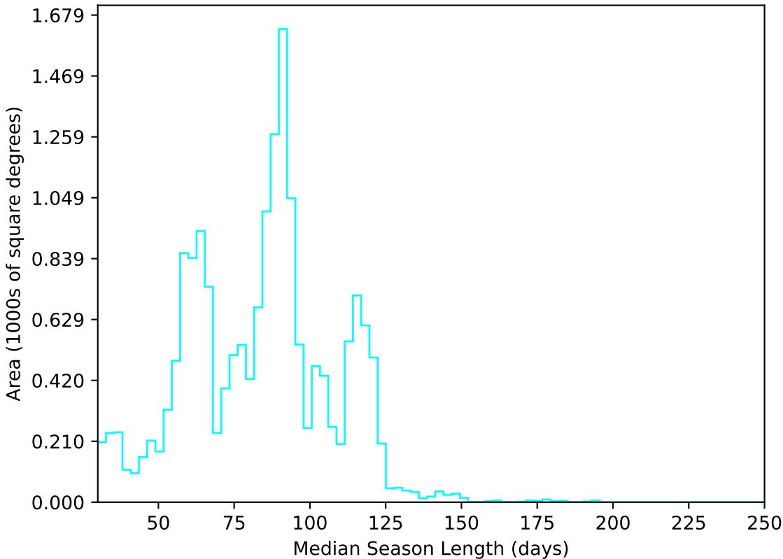
ddf_loaded_half_fl4_v3.4_10yrs WFD u band: Median Season Length
