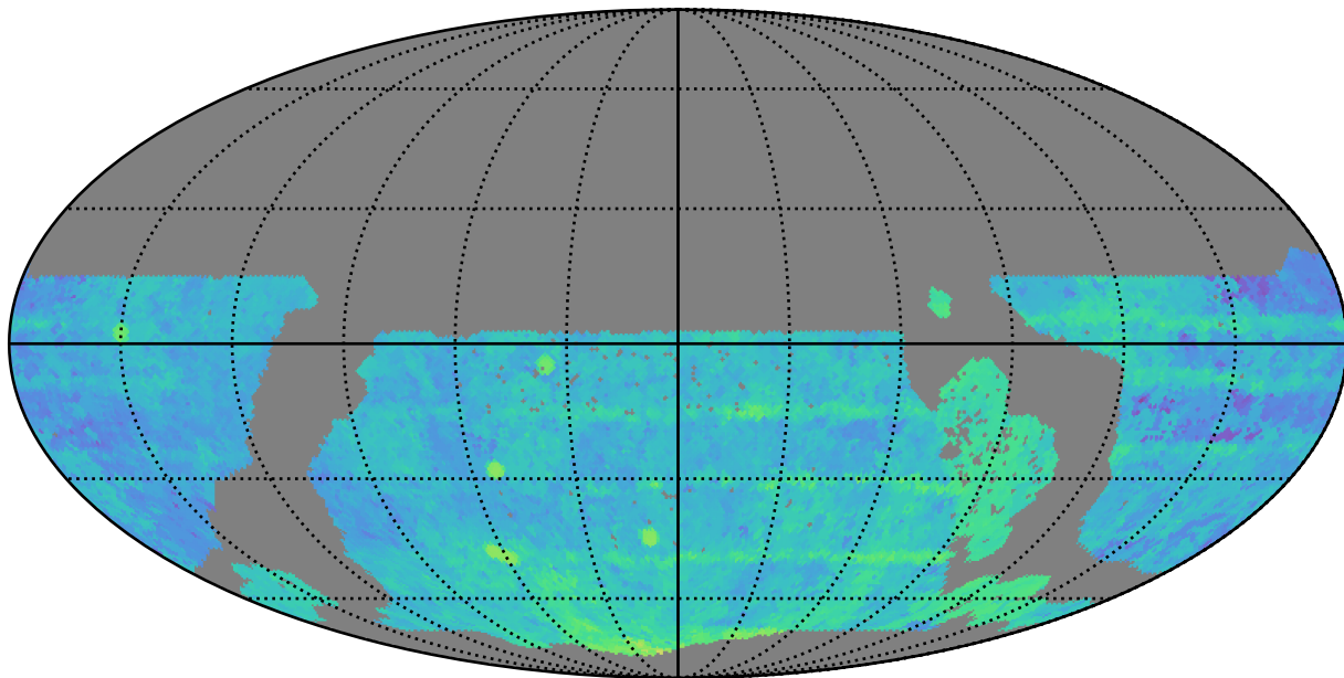
ddf_loaded_half_fl4_v3.4_10yrs WFD r band: Median Season Length
