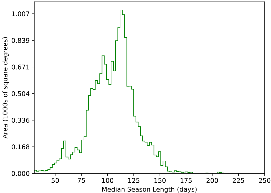
ddf_loaded_half_fl4_v3.4_10yrs WFD g band: Median Season Length
