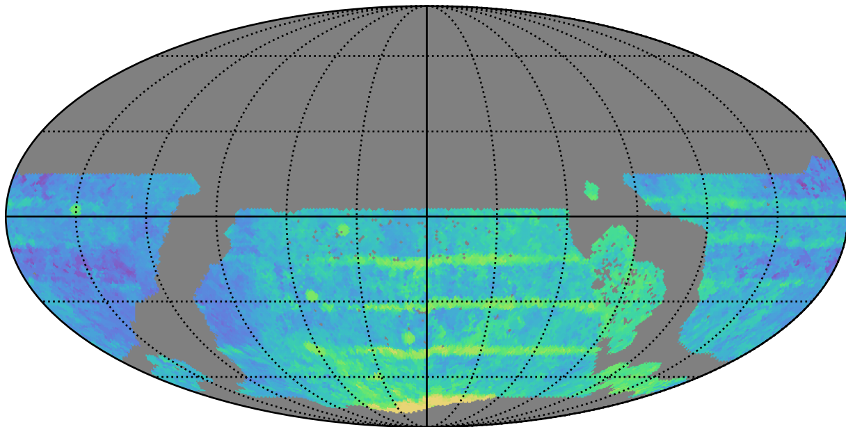
ddf_loaded_half_fl4_v3.4_10yrs WFD all bands: Median Season Length
