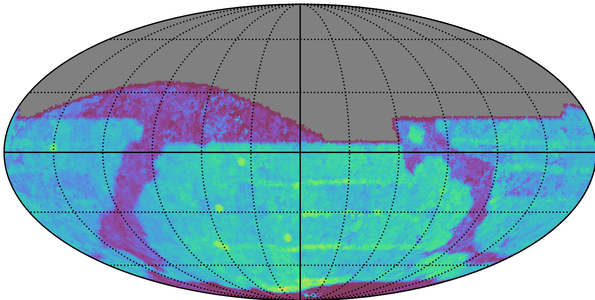
ddf_loaded_half_fl4_v3.4_10yrs All sky z band: Median Season Length
