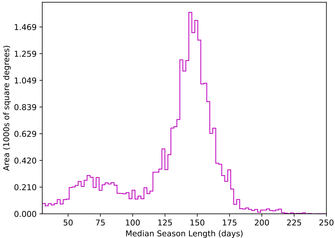
ddf_loaded_half_fl4_v3.4_10yrs All sky z band: Median Season Length
