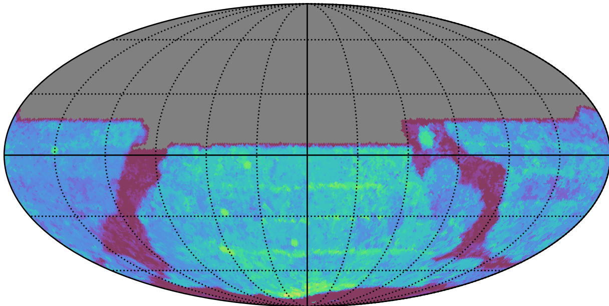
ddf_loaded_half_fl4_v3.4_10yrs All sky y band: Median Season Length
