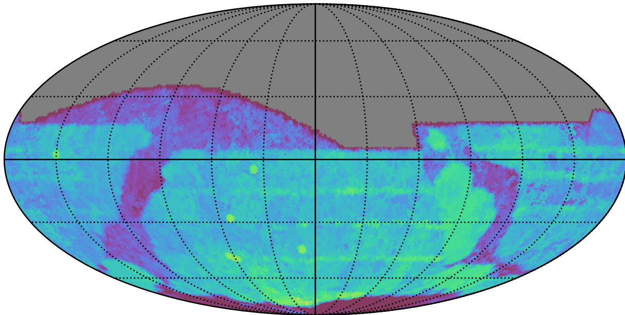
ddf_loaded_half_fl4_v3.4_10yrs All sky r band: Median Season Length
