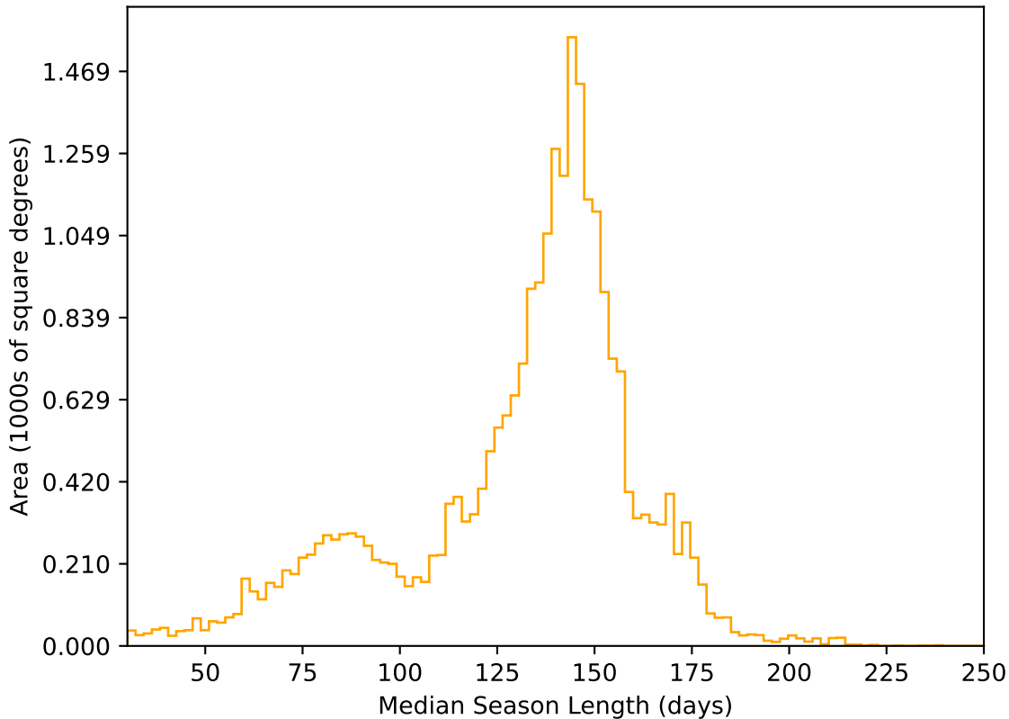
ddf_loaded_half_fl4_v3.4_10yrs All sky r band: Median Season Length
