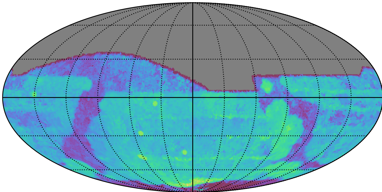
ddf_loaded_half_fl4_v3.4_10yrs All sky i band: Median Season Length
